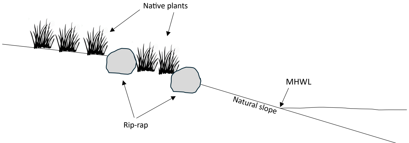
B-3. Tiered rip-rap with planting terrace
