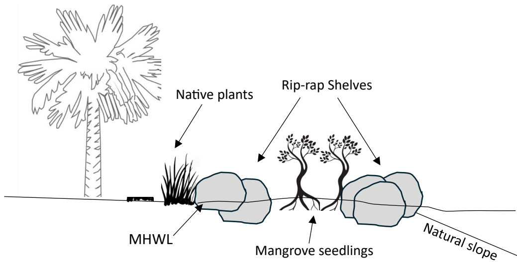
B-4. Rip-rap shelves with native planting
