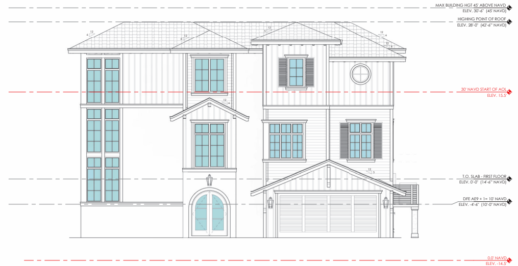
② SOUTH ELEVATION SCALE: 3/16" = 1'-0"
