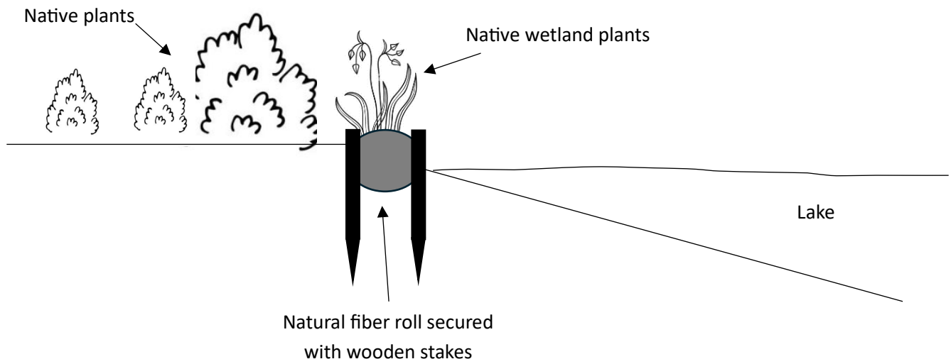
A-3. Natural fiber roll with native planting
