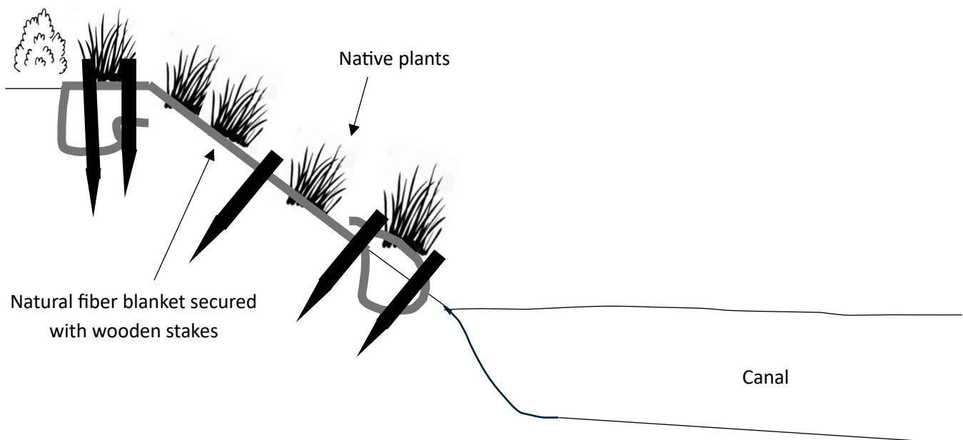
A-4. Native fiber blanket with native planting
