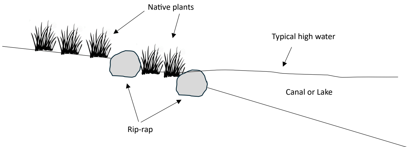
A-2. Tiered rip-rap with planting terrace
